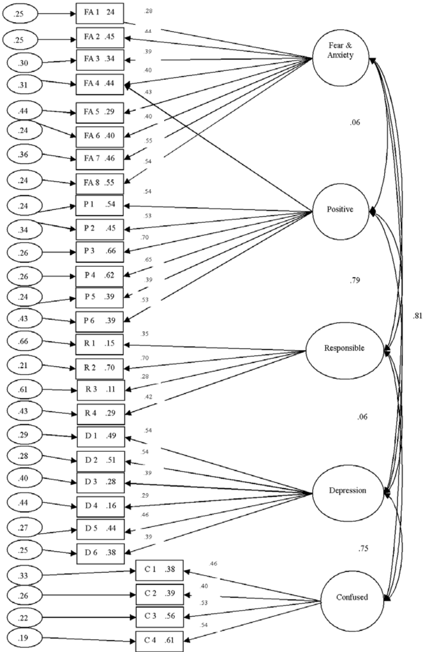
Figure 1 — Path diagram of the 28-item Emotional Reactions to Challenging Behavior Scale-Korean .
