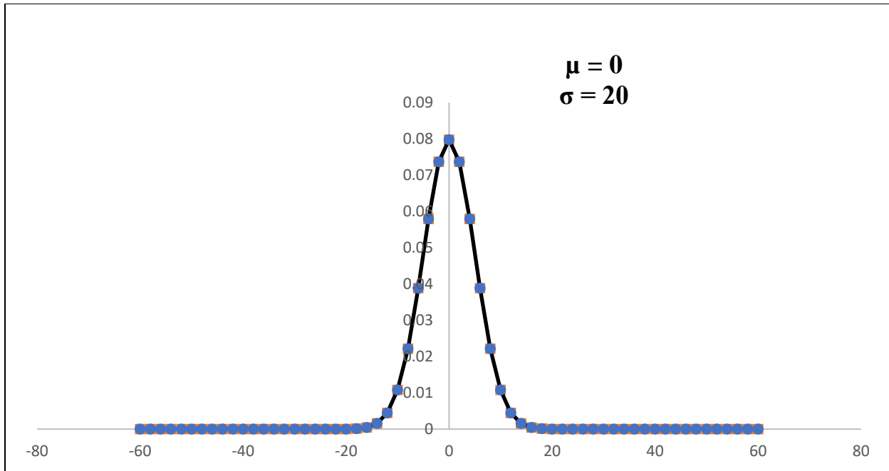
Figure 1. A Normal Distribution with a mean of 0 and standard deviation of 20
