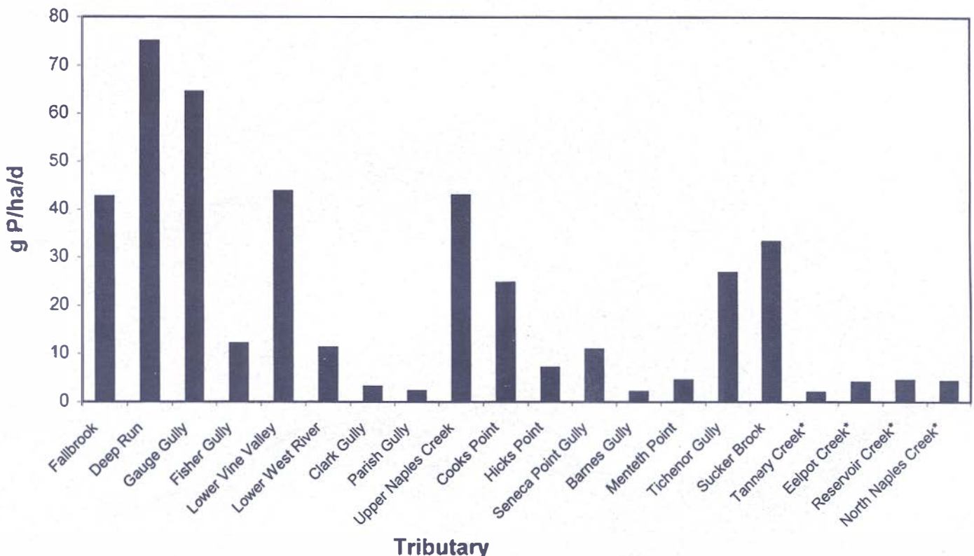
Figure 1. Phosphorus loss from Canandaigua Lake tributaries during precipitation events, 1997-1998 (n=10).
