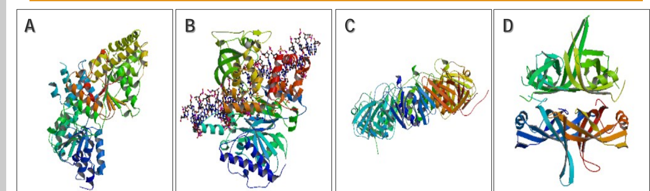
Figure 6: PDB crystal structures of (A) helicase, (B) ligase, (C) polymerase subunit, and (D) single stranded DNA binding protein.
