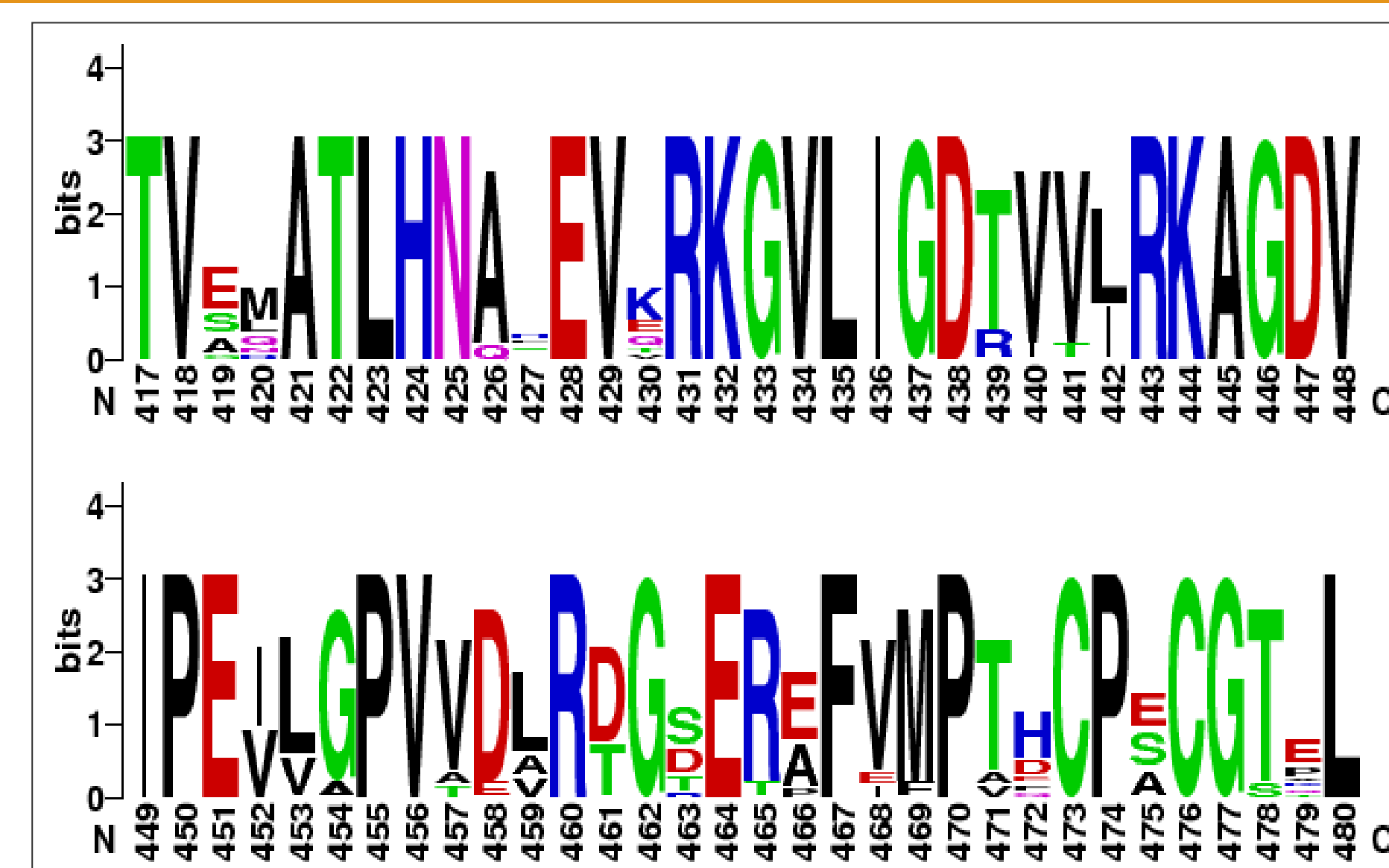
Figure 2: Portion of the WebLogo for gene OID 644991259 showing conservation. The larger the letter the more conservation between the collected homologous sequences and K. sedentarius .
